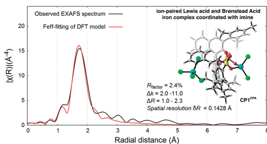
Fourier-transformed Fe K-edge EXAFS spectra in R-space
