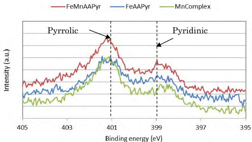
Fig. 3 N1s spectra of HAXPES
