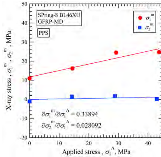
Fig. 8 Change of parallel \sigma_1^m and perpendicular stress \sigma_2^m in PPS under the applied stress \sigma_1^A for GFRP.
