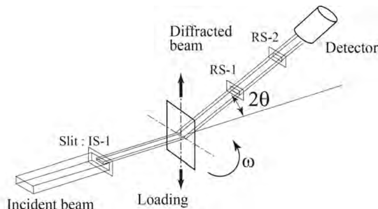
Fig. 1 Experimental set-up.
